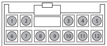
View: Front Side of 12P Connector
