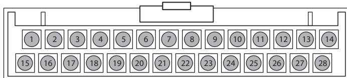
View: Front Side of 28P Connector
