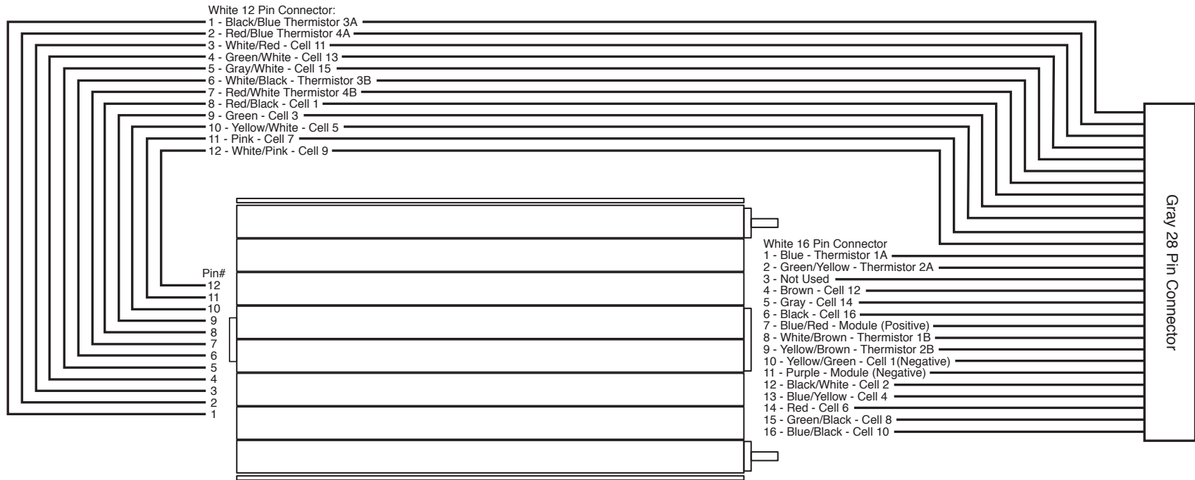
View: Front Side of 12P Connector
