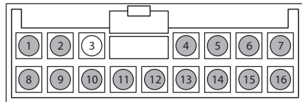
View: Front Side of 16P Connector
