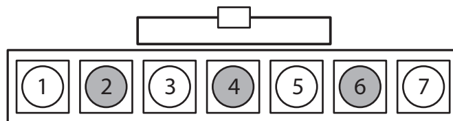
View: Front Side of 7 Pin Battery Connector
