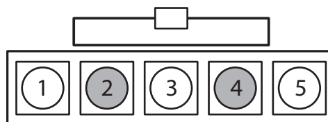
View: Front Side of 5 Pin Battery Connector
