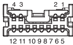
View: Looking at the FRONT Side of the BMS PCB Connector
